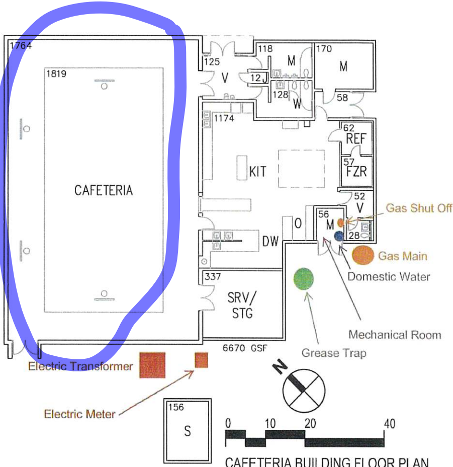
CAFETERIA BUILDING FLOOR PLAN PORTALES JUNIOR HIGH SCHOOL
